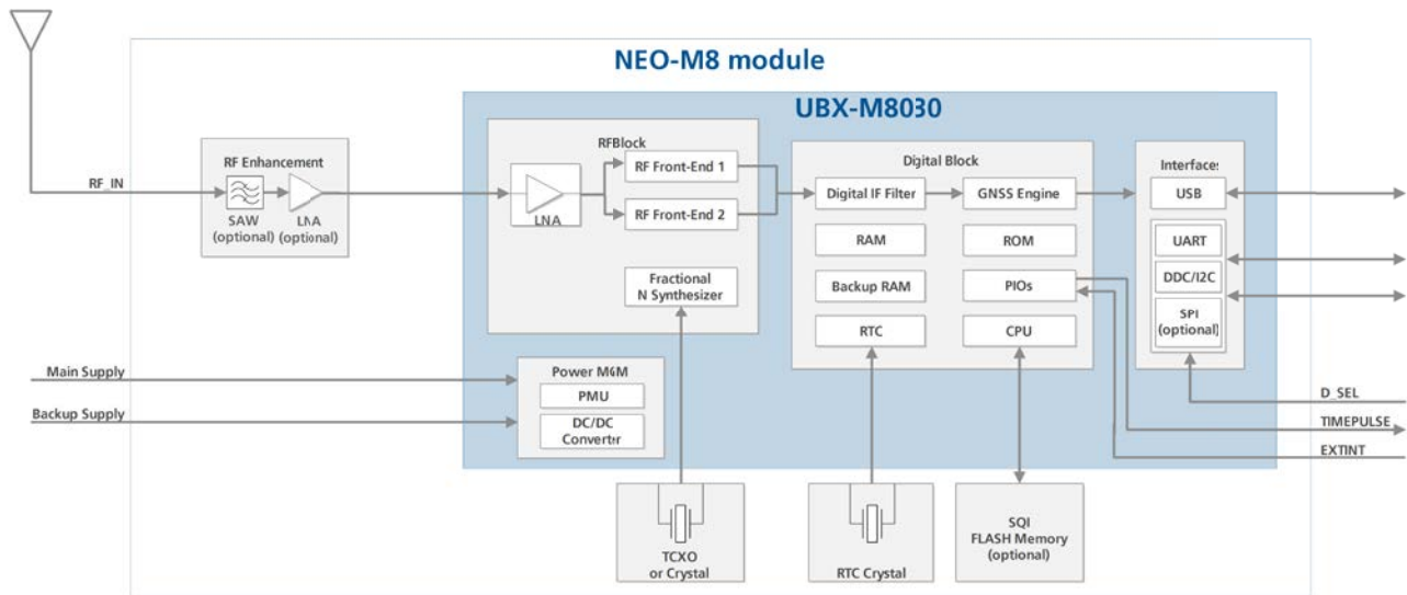
Figure 1: NEO-M8 block diagram
