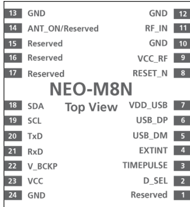
Figure 2: Pin Assignment
